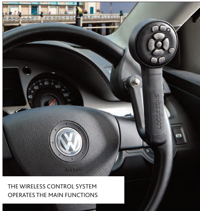
STEERING BALL WITH KEYPAD
